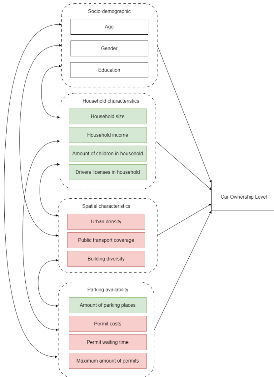
Figure 2. Conceptual model
