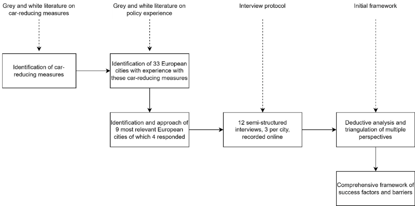
Fig. 1. Research methodology.
